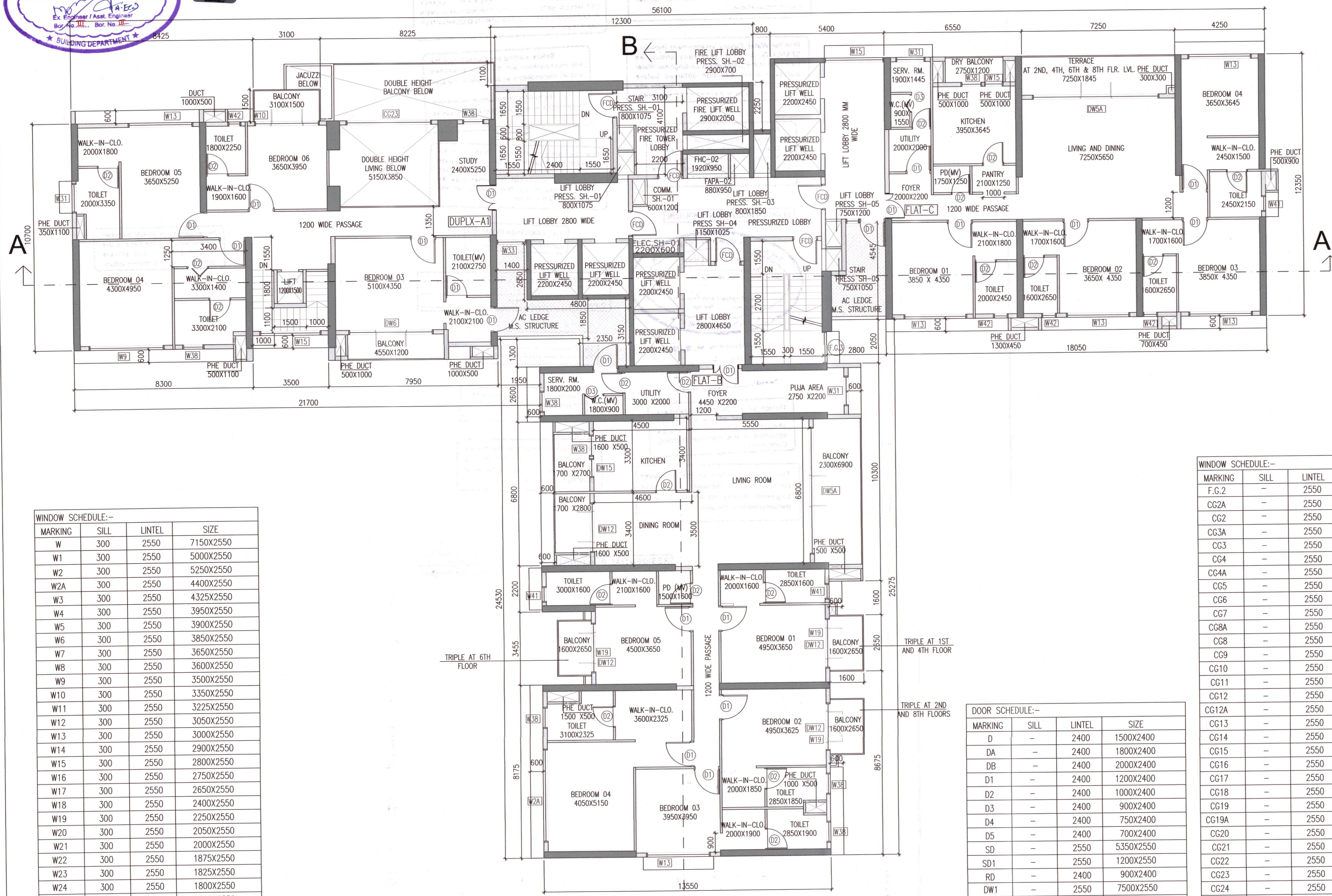
TOWER 2 - 2ND, 4TH, 6TH AND 8TH FLOOR PLAN 1:100
